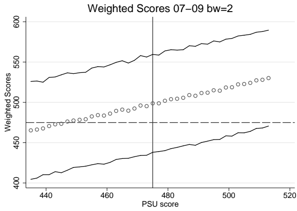
Figure 15: Weighted Score Empirical Distribution.
