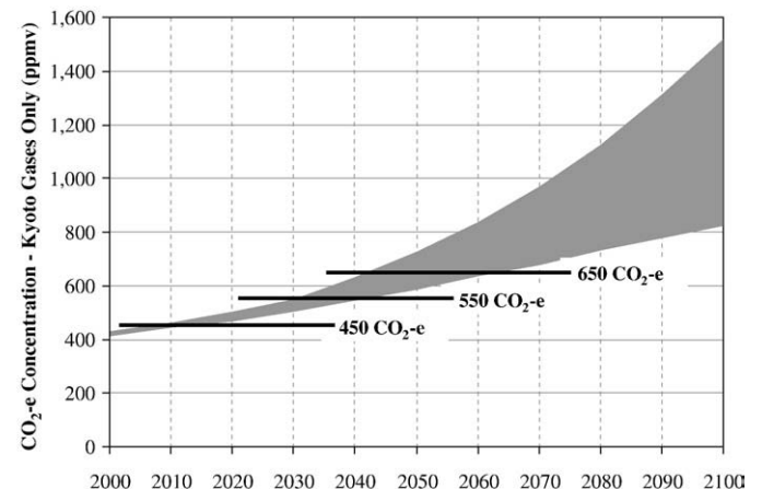
Fig. 2. CO 2 -e concentrations of the Kyoto gases across the EMF 22 reference scenarios.
